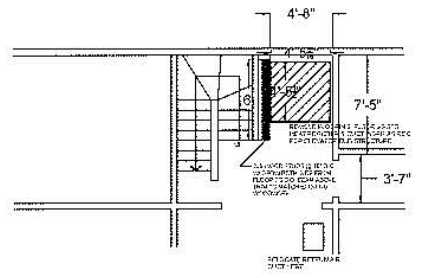
1ST LEVEL PARTIAL FLOOR PLAN 1/8" = 1'-0"
